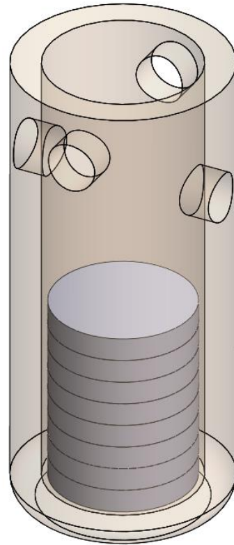
Stacked pellets in crucible
